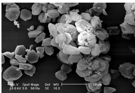
Scanning electron micrographs of the mesoporous silicate MCM-41.
